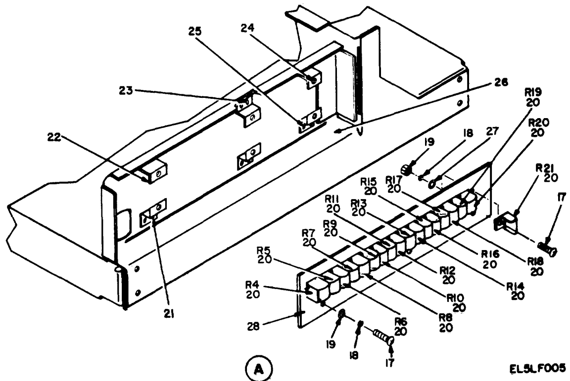
Figure 4. Signal Processor CP-925/TPX-46(V)(1A3), Chassis Top View.
